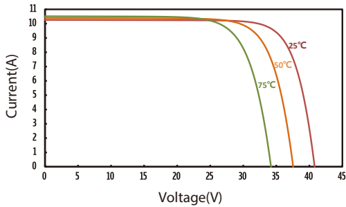
IV Curves of JT330SiH(B) at different Temp
